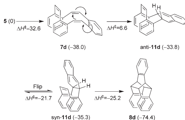
Scheme 3. Computed thermal isomerization of 5 to furnish 8d . \Delta H^\ddagger and ( \Delta H ) values, calculated at the B3LYP/6-31G(d) level, are given relative to 5 (kcal mol -1 ).
